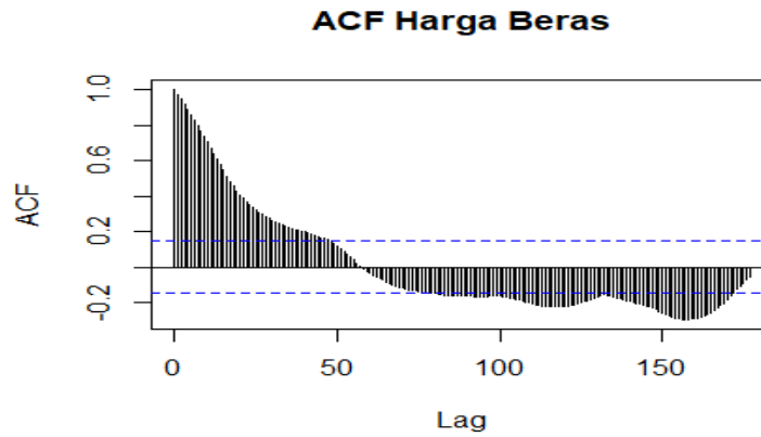
Gambar 4. Plot ACF
