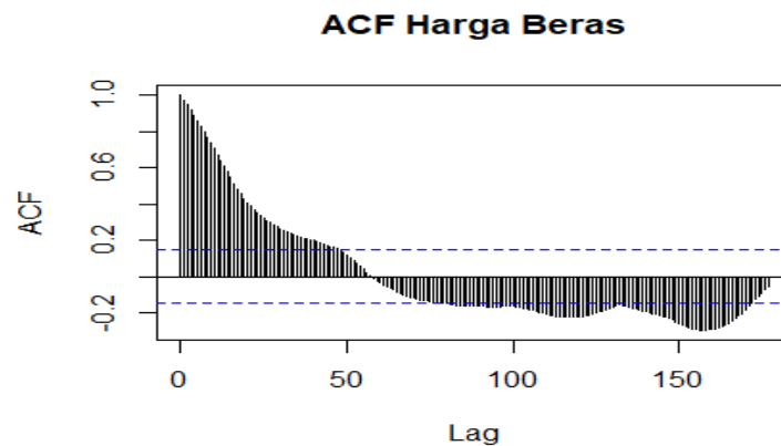
Gambar 3. Plot ACF
